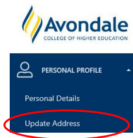
Menu Page
